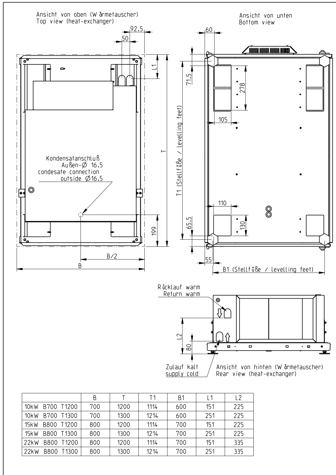
Dimensions bottom plate / cut outs / connections 12- 17 - 25 / 35 kW
